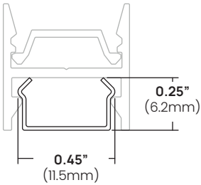
Mounting Clips
