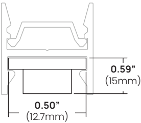
Magnet Mounting
