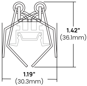
Spring Clip
