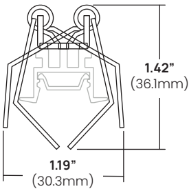
Spring Clips
