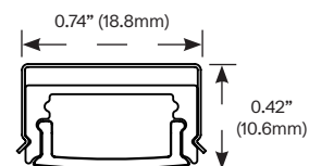
Mounting Clip
